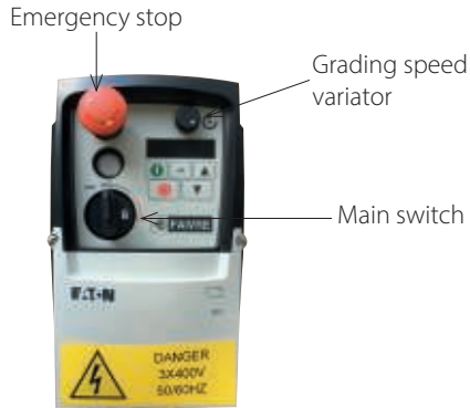
Fish grader IP 67 electric panel.
